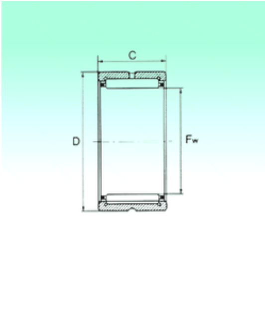
NKS 37 Bearing 2D drawings and 3D CAD models
